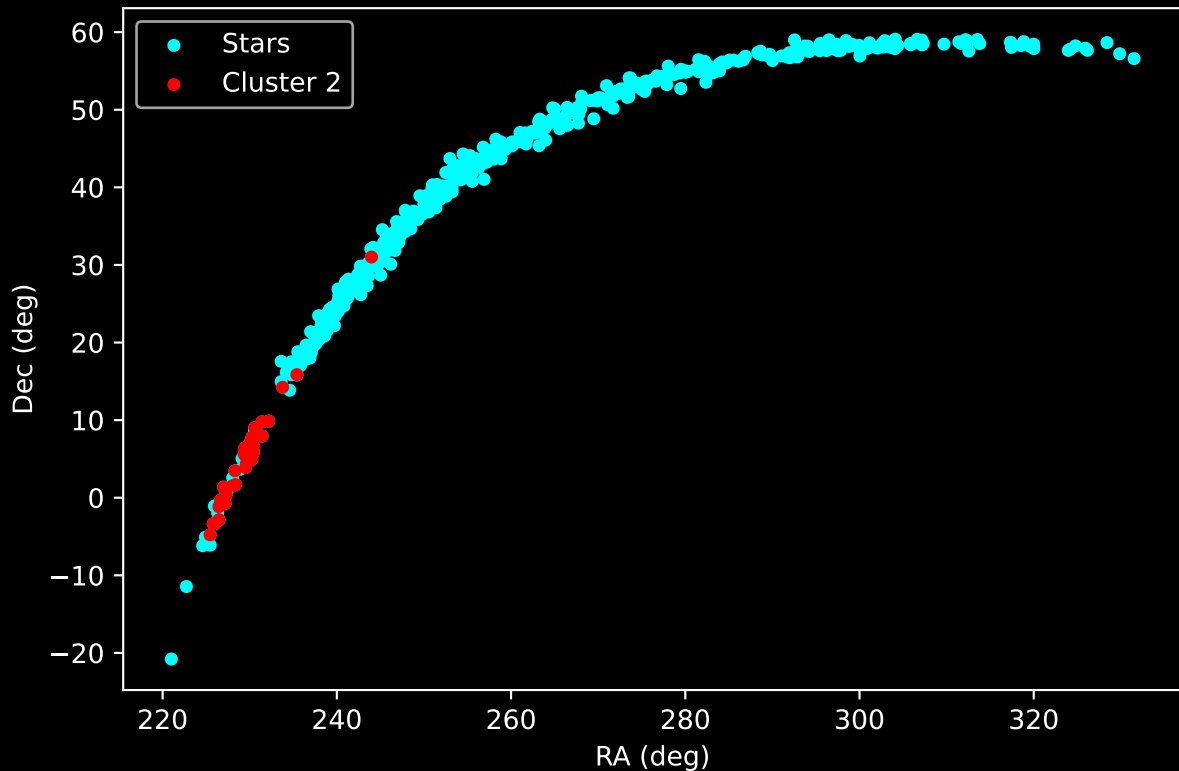
Gaia Stream: [GD-1] Cluster 2 (n= 33) Southern segment, near progenitor search region
